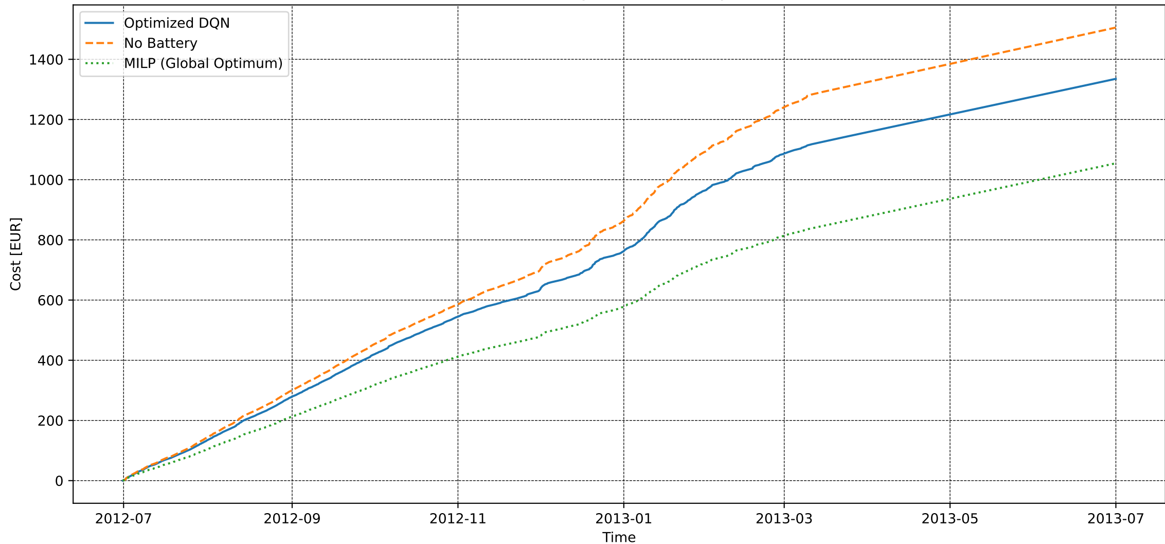
User 138 - Extended Convergence - Electricity Cost [DQN vs MILP]
